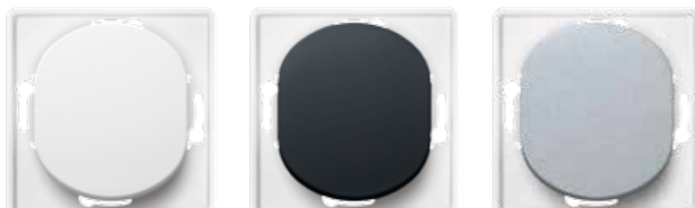
E6052.x Sklopka dvopolna 10AX/250V~ Double-pole switch 10AX/250V~
