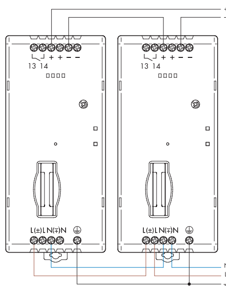
Series connection
