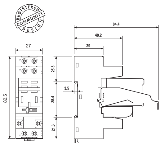
96.02 96.02 + 56.32 + 094.91.3 + 86.30
