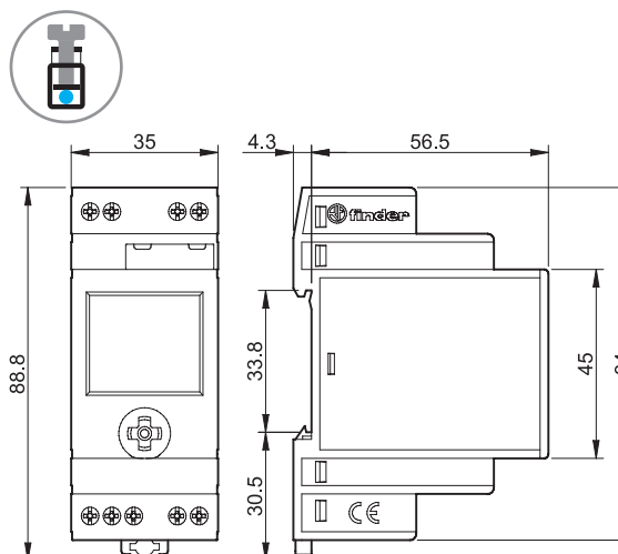
11.91 Screw terminal
