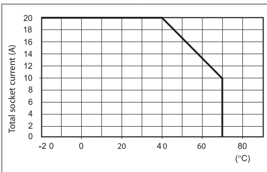
L 95 - Total socket current v ambient temperature
