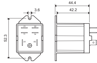
065.05 with relay
