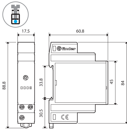
14.91 Screw terminal
