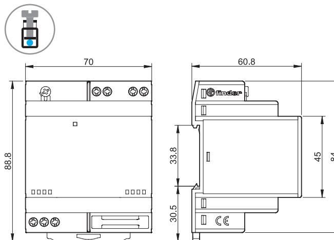
78.51 / 78.61 Screw terminal
