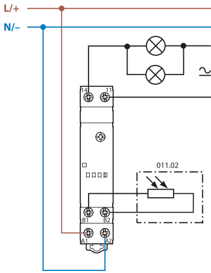
Type 11.42
