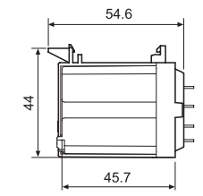
062.08 with relay
