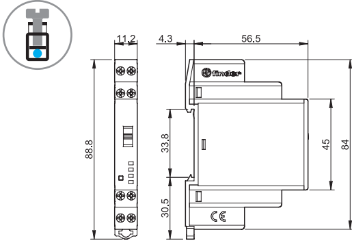
Type 19.21 Screw terminal
