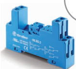
95.85.3 See page 9
