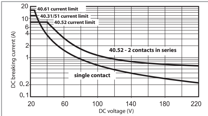
H 40.1 - Maximum DC1 breaking capacity
