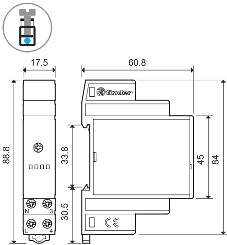
14.81 Screw terminal
