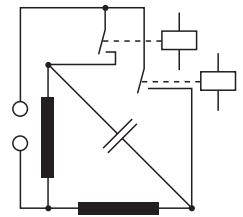
Correct AC motor reversal:
