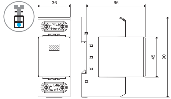
Type 7P.01 Screw terminal
