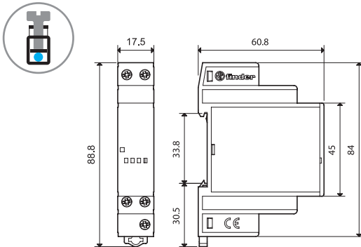
Type 19.91 Screw terminal
